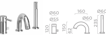
3TH BATH SET
