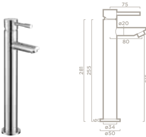
TALL BASIN MONO
