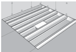
1 Cut out required section of flooring and fix battens to joists
